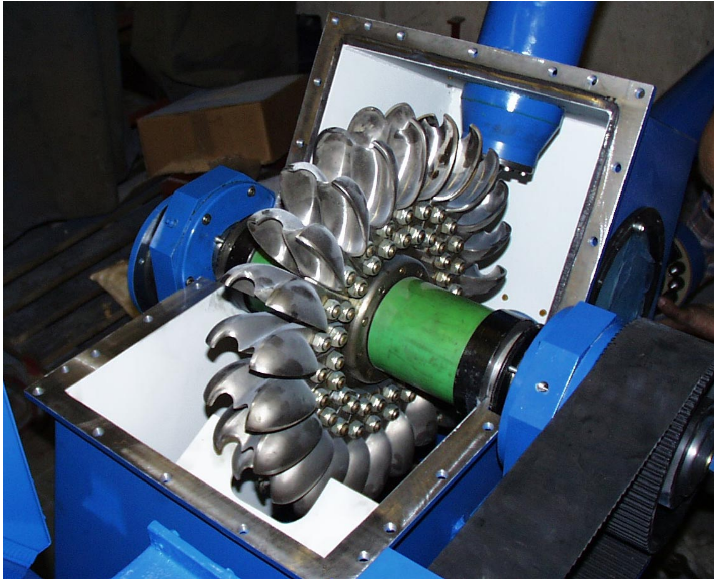
Pelton Wheel
