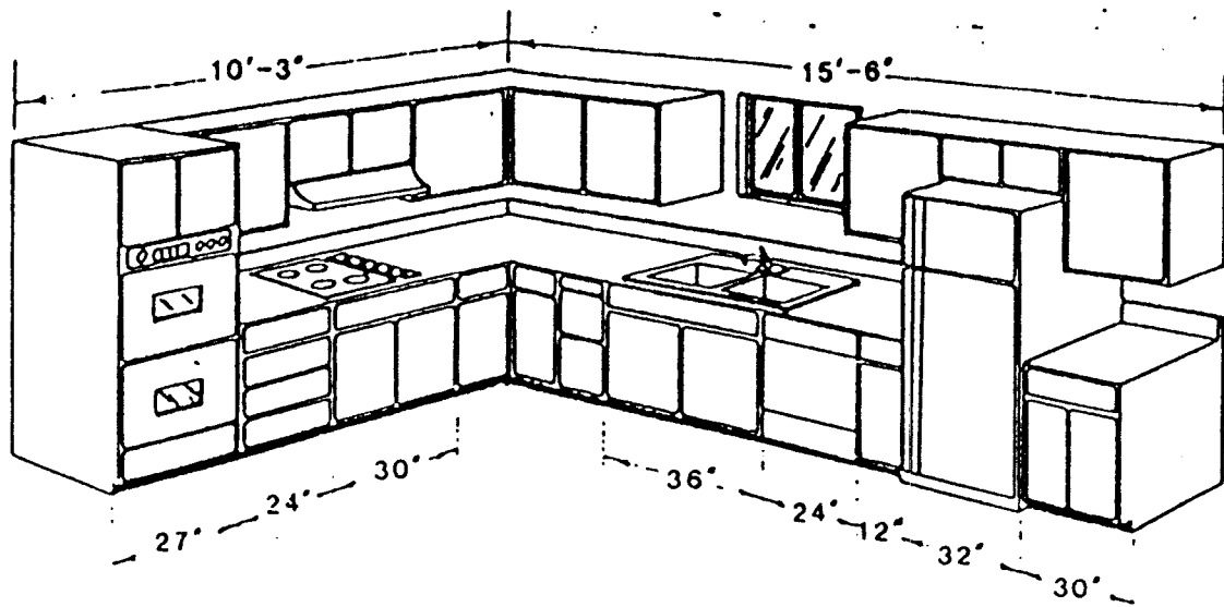
Fig. 16-17 Design standards for modular kitchen units. (William Wagoner)
