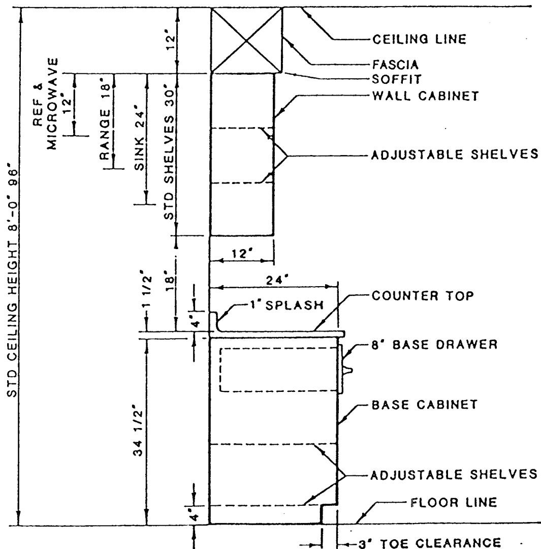
Fig. 16-18 Wall and base cabinet standard dimensions.
